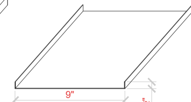
OS-912SP - 1/2"D x 9"W Splice
